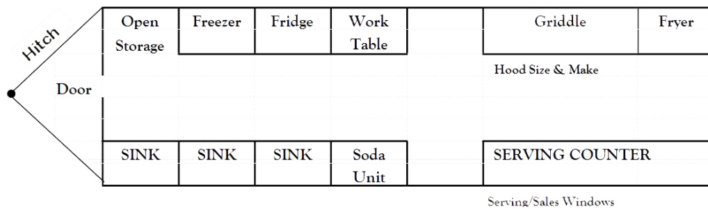
8.5'x18' CUSTOM CONCESSION TRAILER SAMPLE FLOORPLAN
