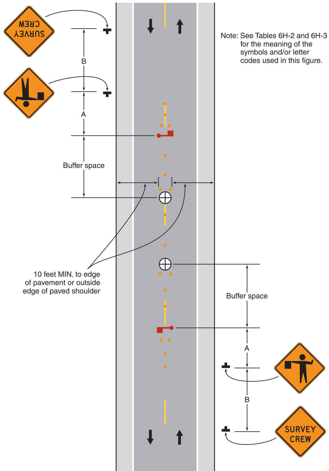
Typical Application 16
