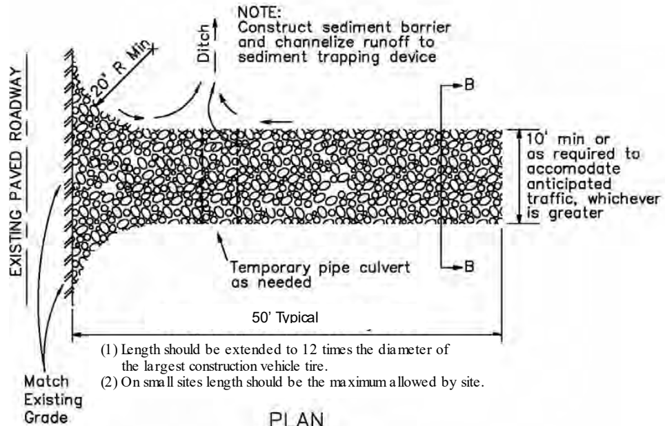
PLAN NTS
